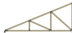
Mono truss
