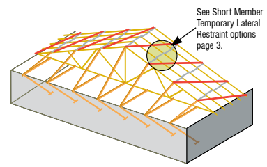
INTERIOR GROUND BRACING TO END WALL ARRIOSTRE DE TIERRA INTERIOR A LA PARED DE EXTREMO
